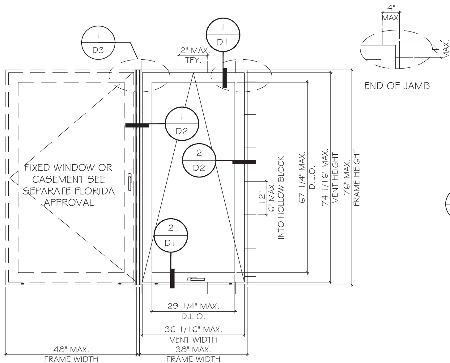
TYPICAL EXTERIOR ELEVATION
